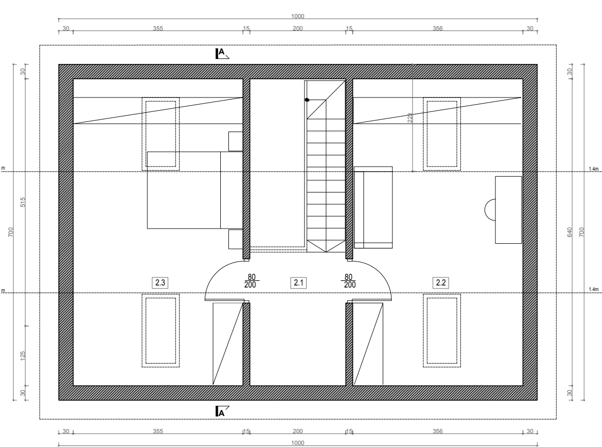
VARIATION 1_USABLE ATTIC PLAN
